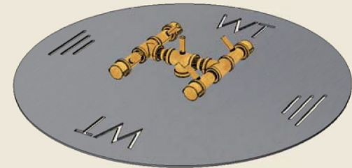
MLS60 - Match Lit 60K System shown with 24" round plate. Other plate options available
