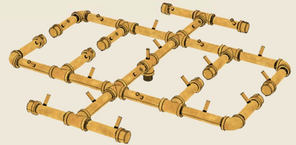
CFB300 - Crossfire 300K System shown with Natural Gas Jets. Liquid Propane also available
