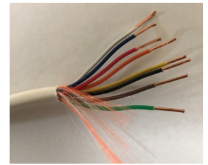
56489901 White Jacket, Non-Shielded Plenum 18AWG Solid 8 Conductor Available in 250' reel
