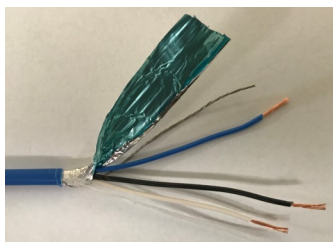
WCW-22/3BLU-WC-S BACnet Communications wire Blue Jacket, Shielded 22AWG Stranded 3 Conductor Available in 500' and 1000' reels
