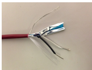
0043280ALR-S Alerton / BACnet Communications wire Raspberry Jacket, Shielded 22AWG Stranded 2 Conductor Available in 500' and 1000' reels
