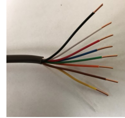
84207 Brown Jacket, Non-Shielded Non-plenum 18AWG Solid 7 Conductor Available in 250' reel
