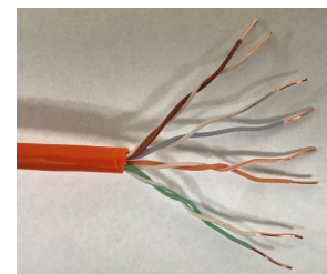
5556140-S Ethernet Communications wire CAT5E Orange Jacket, Non-Shielded 24AWG Solid 4 Pair 8 Conductor Available in 500' and 1000' reels
