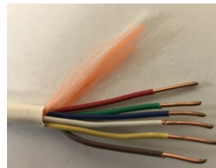
56489601 White Jacket, Non-Shielded Plenum 18AWG Solid 6 Conductor Available in 250' reel
