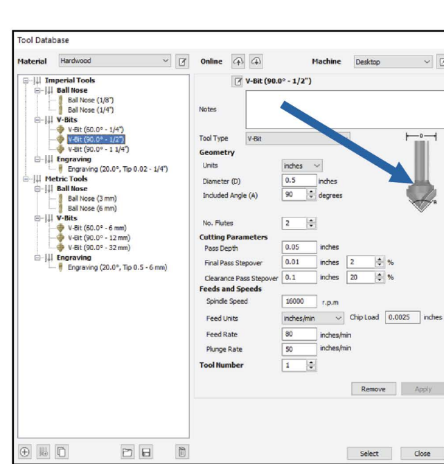
6 Select a router bit, set the feed, cutting depth and router speed
