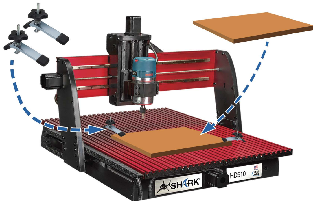
8 Clamp your material to the CNC
