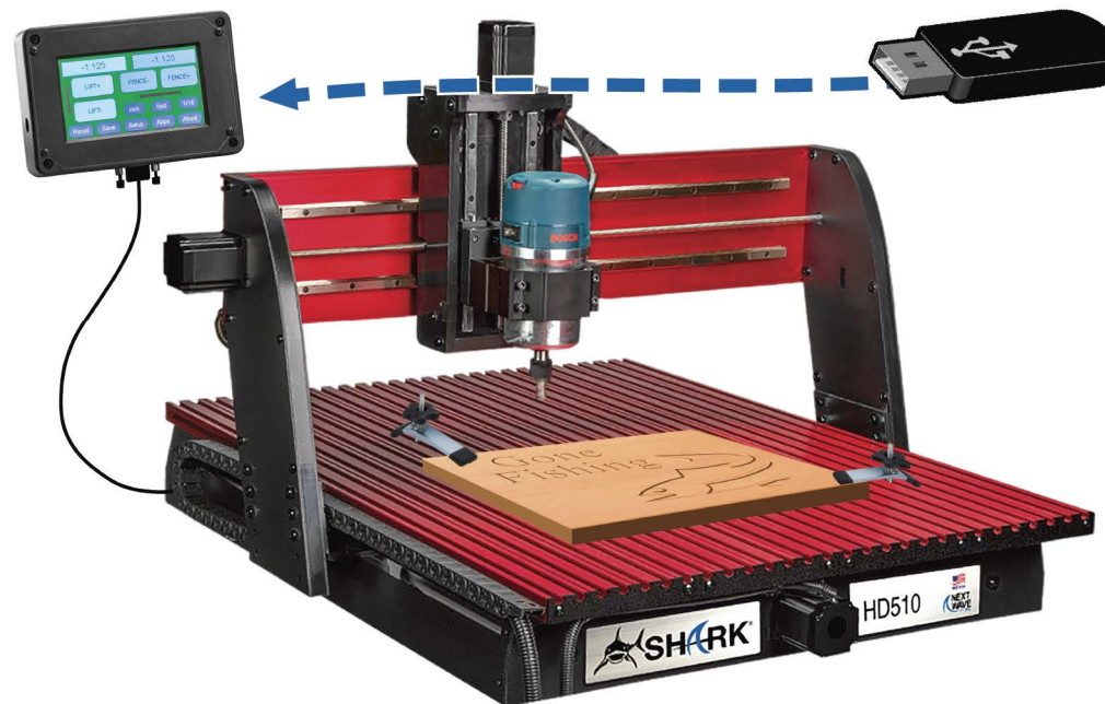
9 Insert thumb drive into the Pendant and rout your design
