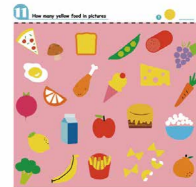
Color recognition
