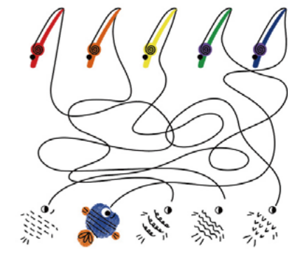
Logic learning
