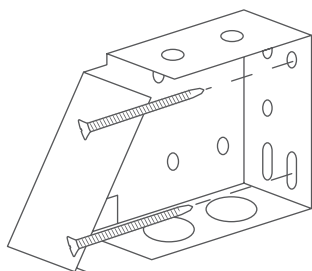
FIG 1.1 Brackets are installed on surface of wall or window frame.
