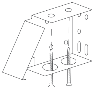
FIG 1.2 Located top inside of the window frame (inside mount) or to the ceiling (outside mount).
