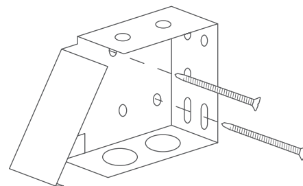
FIG 1.3 Most common for mounting within the window frame (inside mount order).
