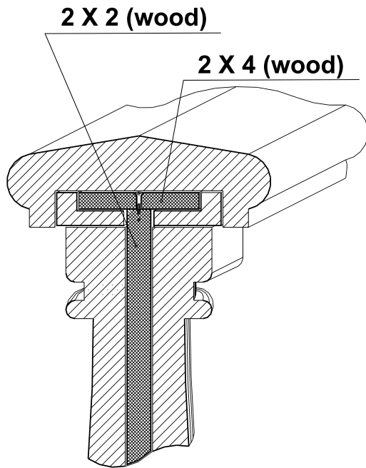
Balustrade system installation
