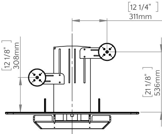
Max/Min Dual Screen Height and Offset
