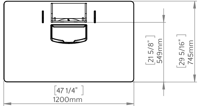
Platform Depth, Block
