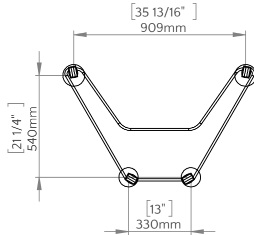
Wheel to Wheel Dimensions (centre)
