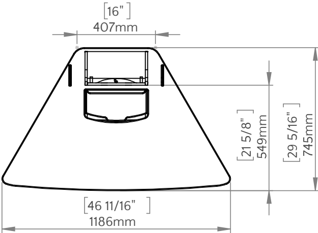
Platform Depth, Petal
