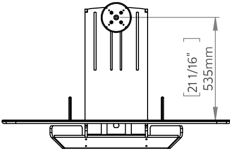
VESA - Maximum Standard Height, Single
