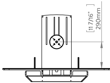
VESA - Minimum Standard Height, Single
