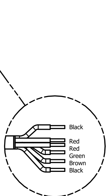
DETAIL C SCALE 1 / 1.5
