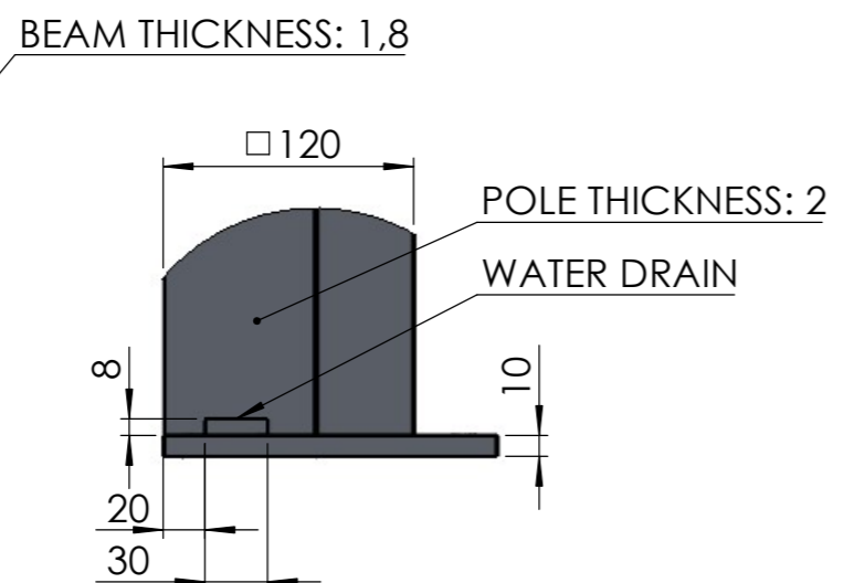
DETAIL B
