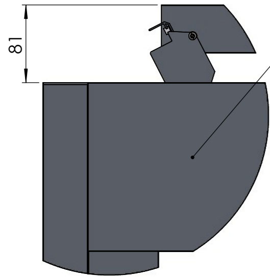
DETAIL A OPEN POSITION
