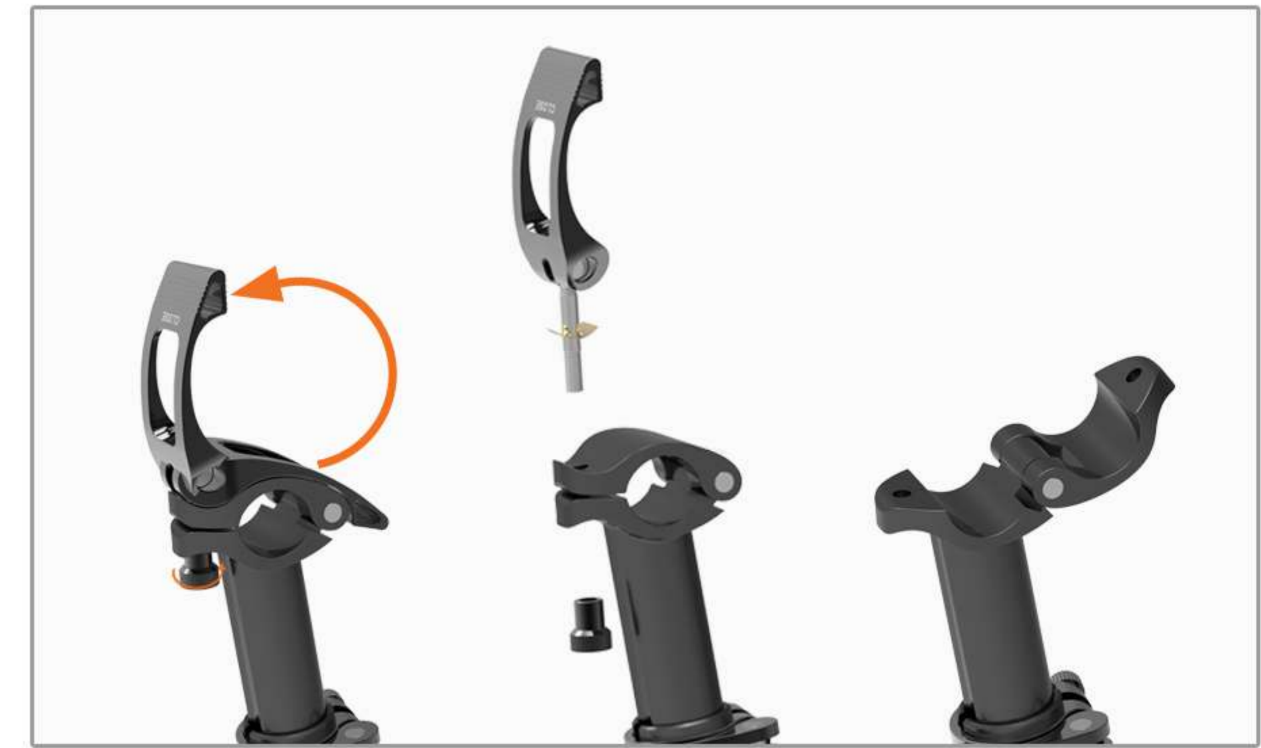
03 Remove the quick release lever from the handlebar, open the handlebar and install the valve cover
