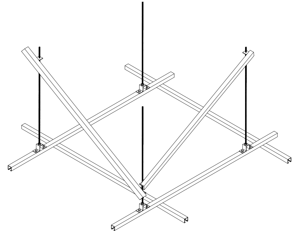
TYPICAL GRID-PARTIAL ISOMETRIC NOT TO SCALE
