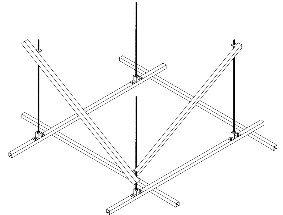
TYPICAL GRID-PARTIAL ISOMETRIC NOT TO SCALE NOE: ISOMETRIC VIEW IS FOR REFERENCE ONLY, AND MAY NOT MATCH THE THE PART NUMBER SHOWN
