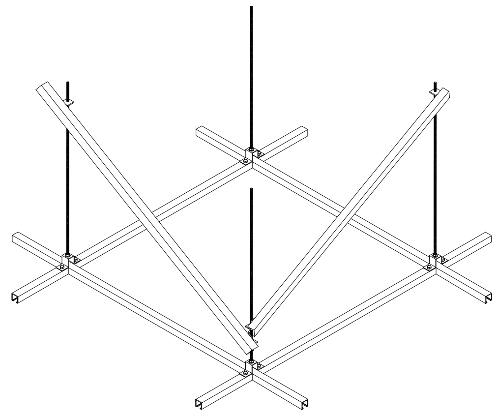
TYPICAL GRID-PARTIAL ISOMETRIC NOT TO SCALE
