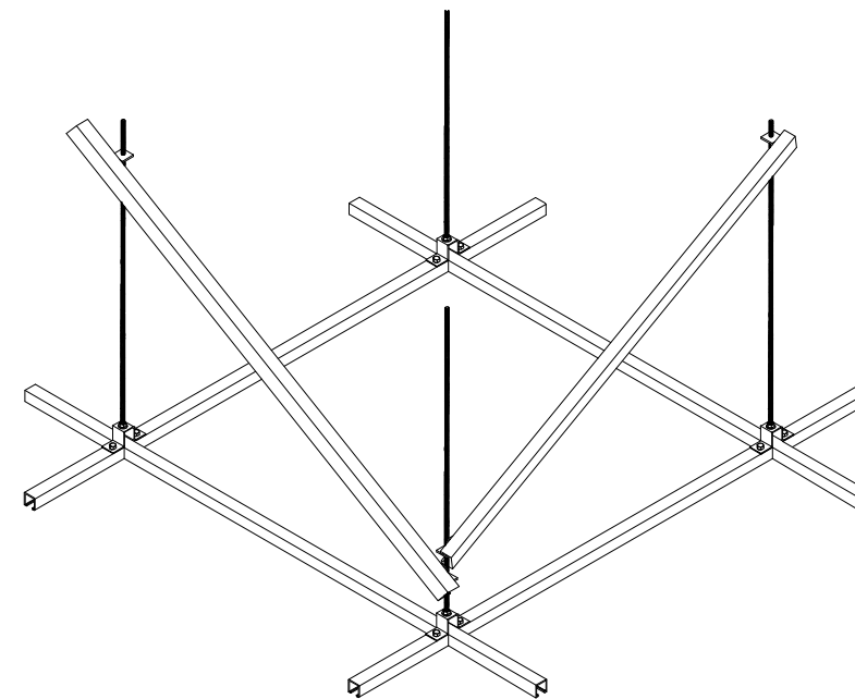
TYPICAL GRID-PARTIAL ISOMETRIC
