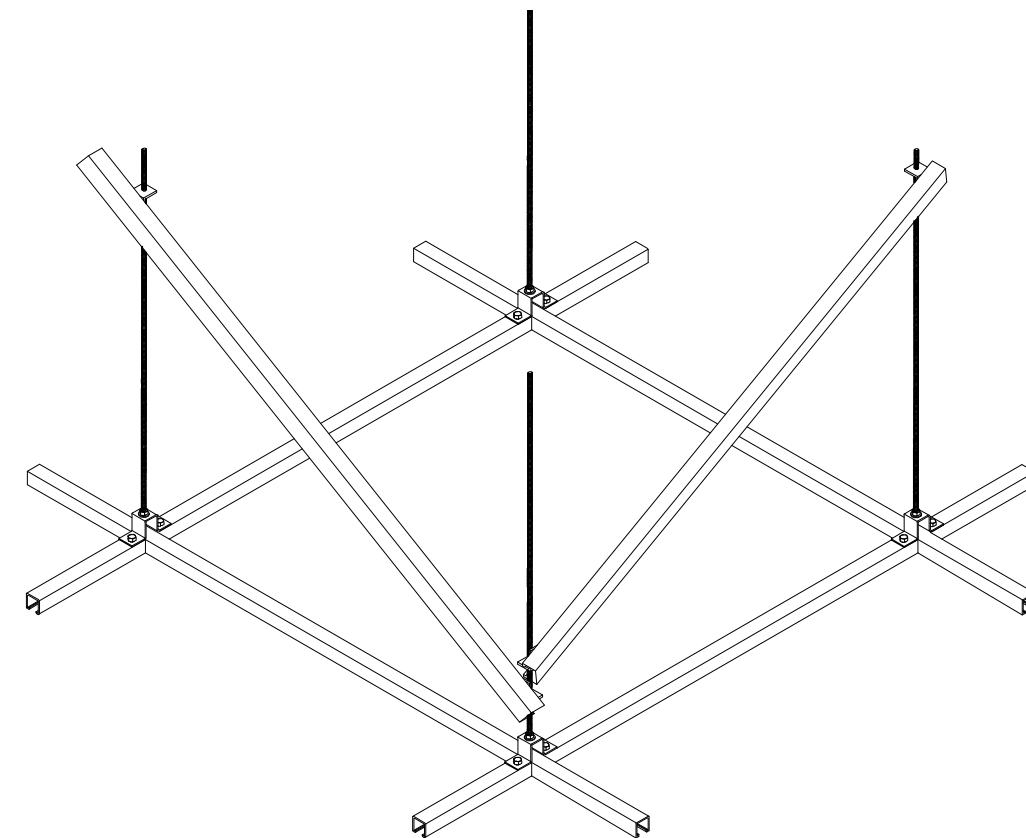
TYPICAL GRID-PARTIAL ISOMETRIC
