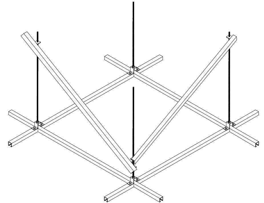
TYPICAL GRID-PARTIAL ISOMETRIC NOT TO SCALE NOE: ISOMETRIC VIEW IS FOR REFERENCE ONLY, AND MAY NOT MATCH THE THE PART NUMBER SHOWN
