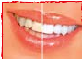
Bleaching
