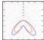
LED 70W Real light output - 4482 lm CRI > 80
