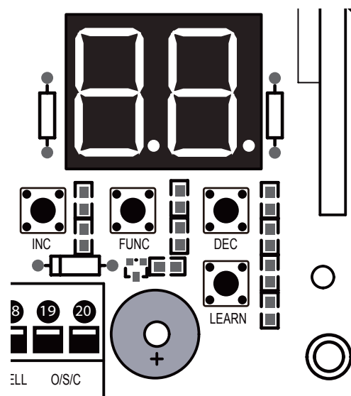
Control Board of KD Series Swing Gate Opener
