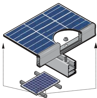
Figure 21. Mounting hole installation example
