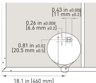
Figure 19. Mounting holes_EVPVxxxH Series modules
