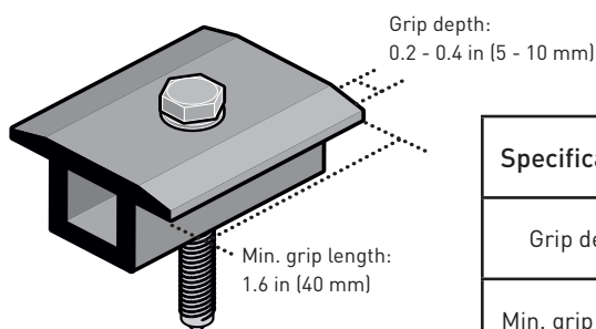
Figure 7. Clamp specifications
