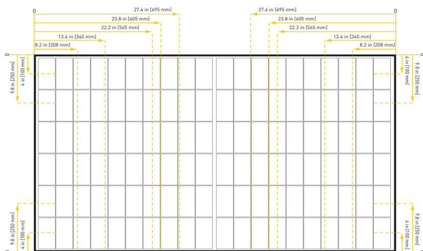
Figure 11. Clamping of EVPVxxx and EVPVxxxK Series modules using short rails
