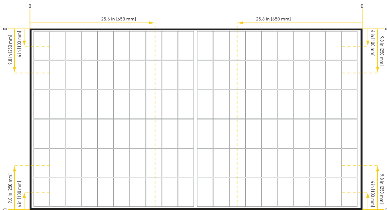
Figure 10. Clamping of EVPVxxx and EVPVxxxK Series modules with rails parallel to long side of the module
