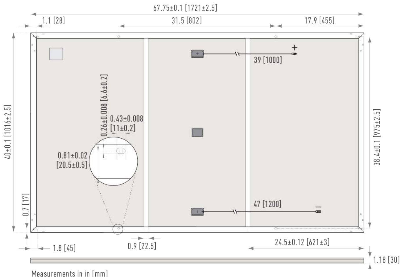
Figure 1. Module Dimension for EVPVxxx and EVPVxxxK Series and EVPVxxxHK Series
