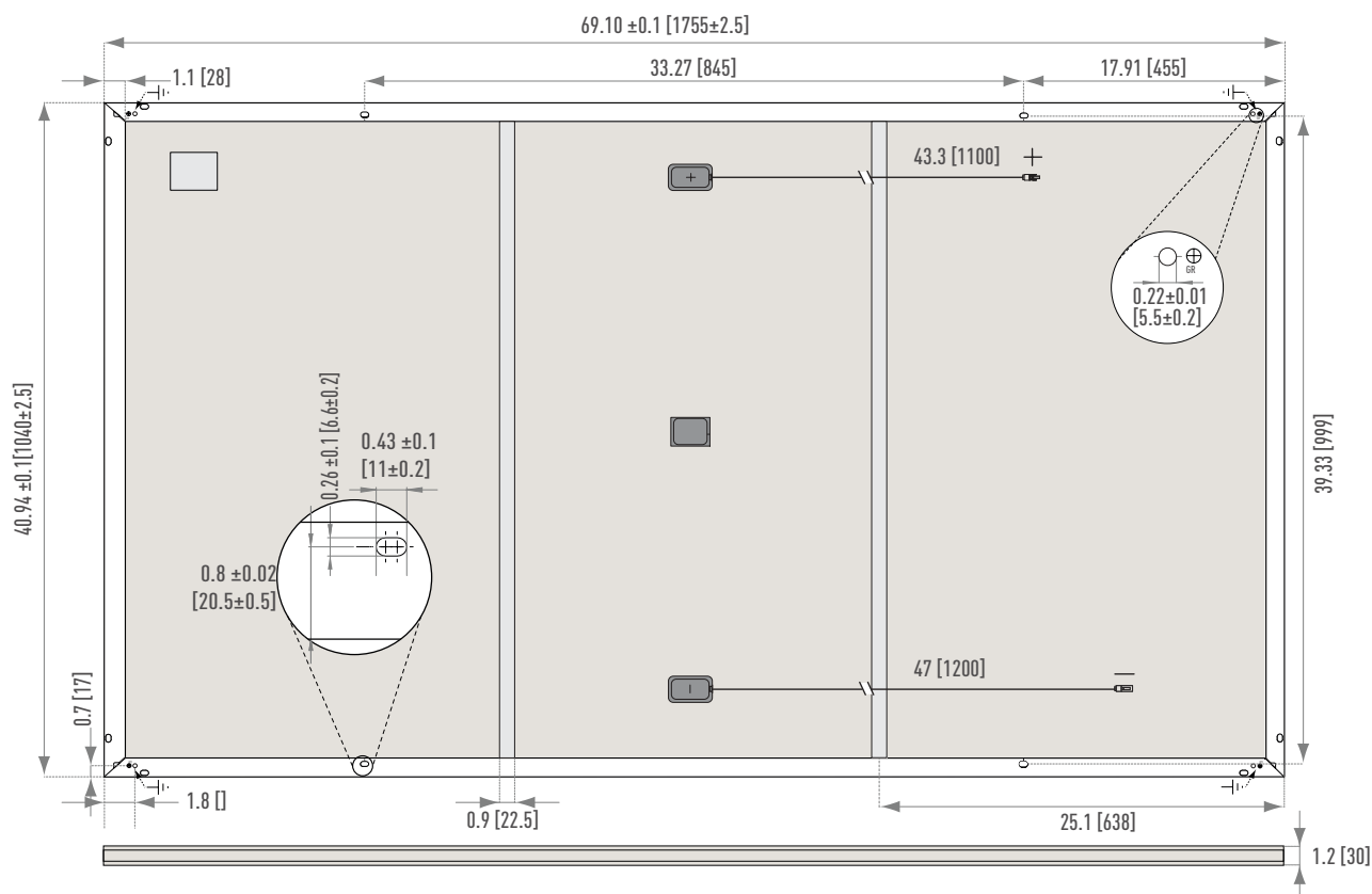
Figure 3. Module Dimension for EVPVxxxPK Series
