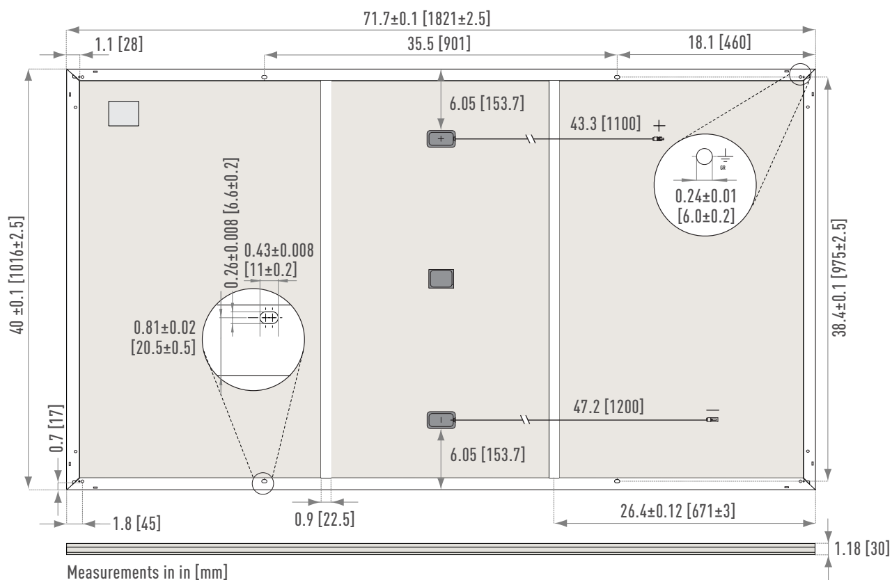
Figure 2. Module Dimension for EVPVxxxH and EVPVxxxHK Series
