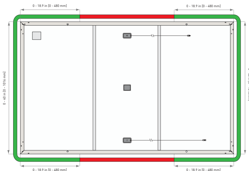
Figure 24. MLPE device installation zones
