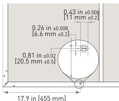
Figure 18. Mounting holes_EVPVxxx, EVPVxxxK, EVPVxxxPK Series modules
