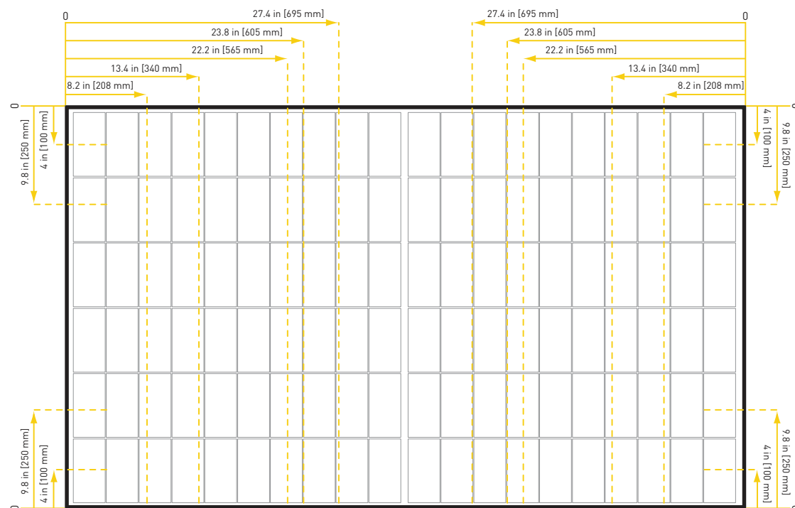
Figure 9. Clamping of EVPVxxx and EVPVxxxK Series modules with rails parallel to short side of the module
