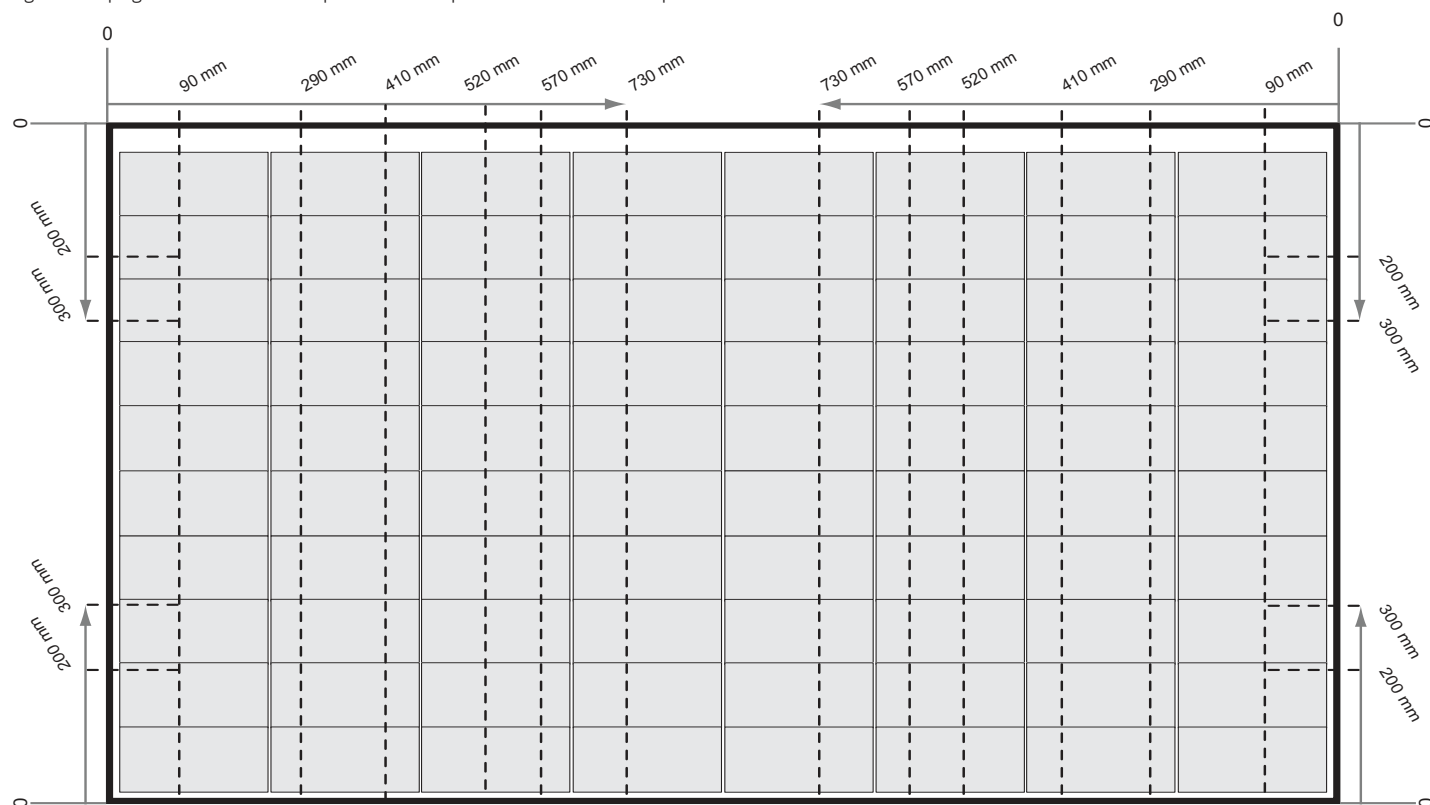
Fig. 9: Clamping of REC Pure-RX Series panels with rails parallel to short side of the panel
