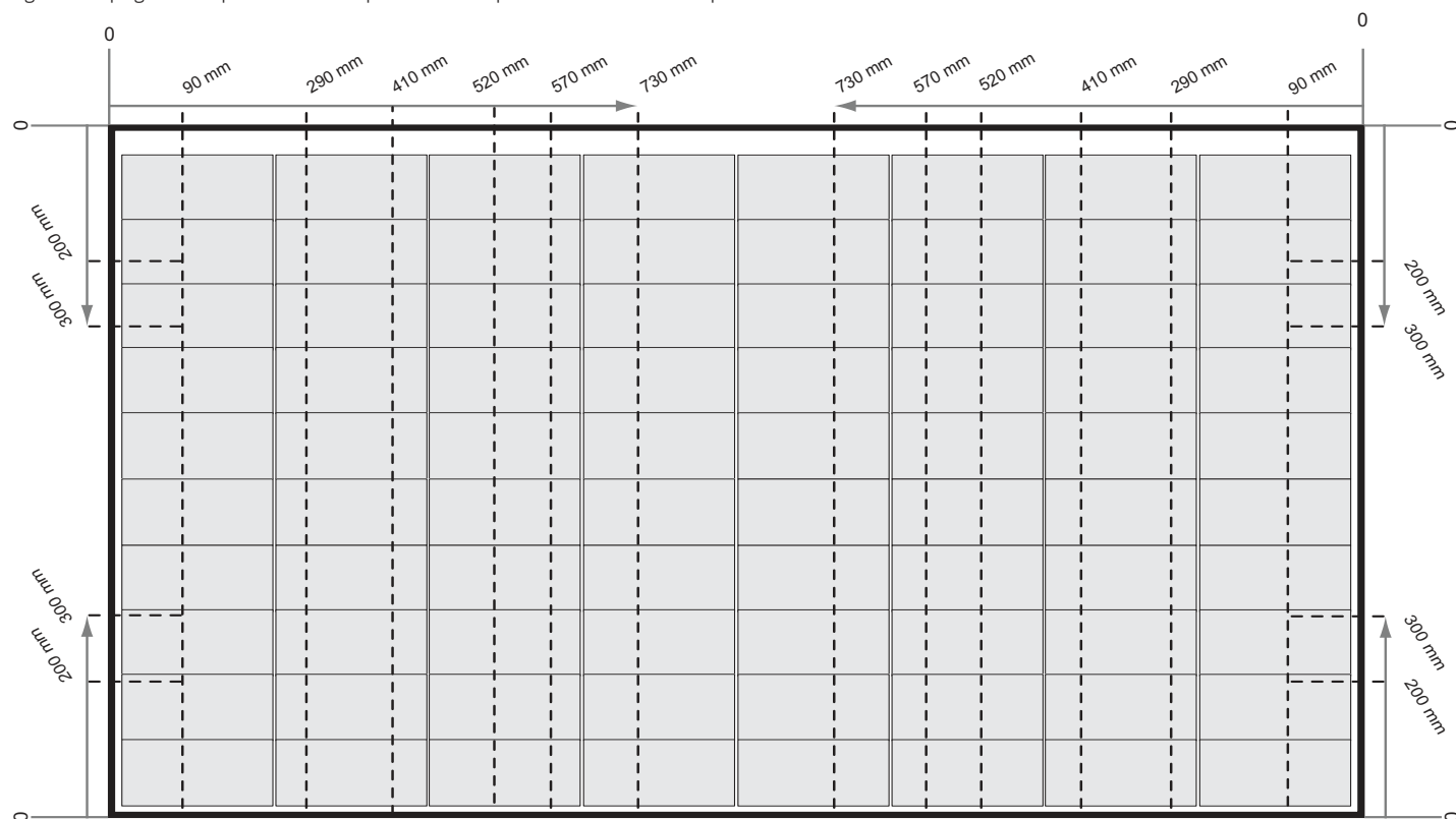
Fig. 6: Clamping of REC Alpha Pure-R Series panels with rails parallel to short side of the panel
