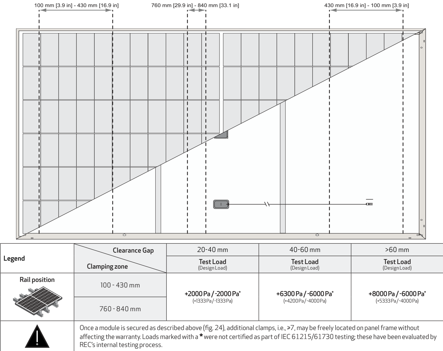
Fig. 15: Six-point mounting configuration clamping zones: REC Alpha Pure Series
