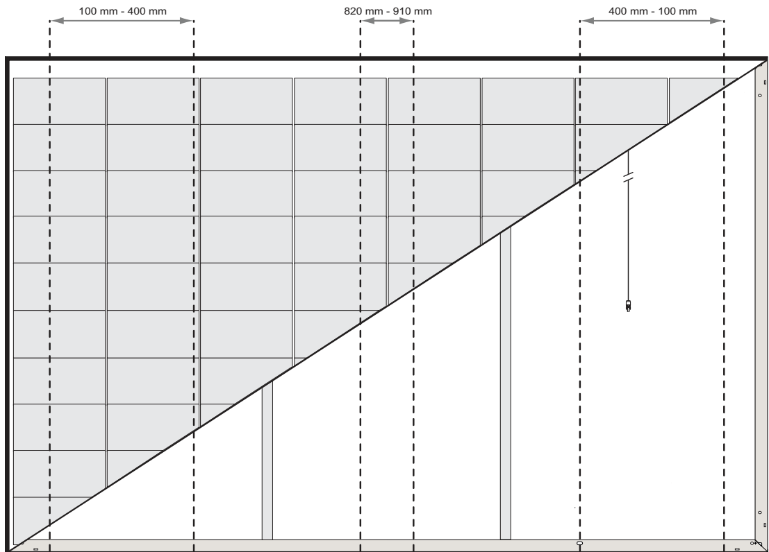
Fig. 16: Six-point mounting configuration clamping zones: REC Alpha Pure-R Series
