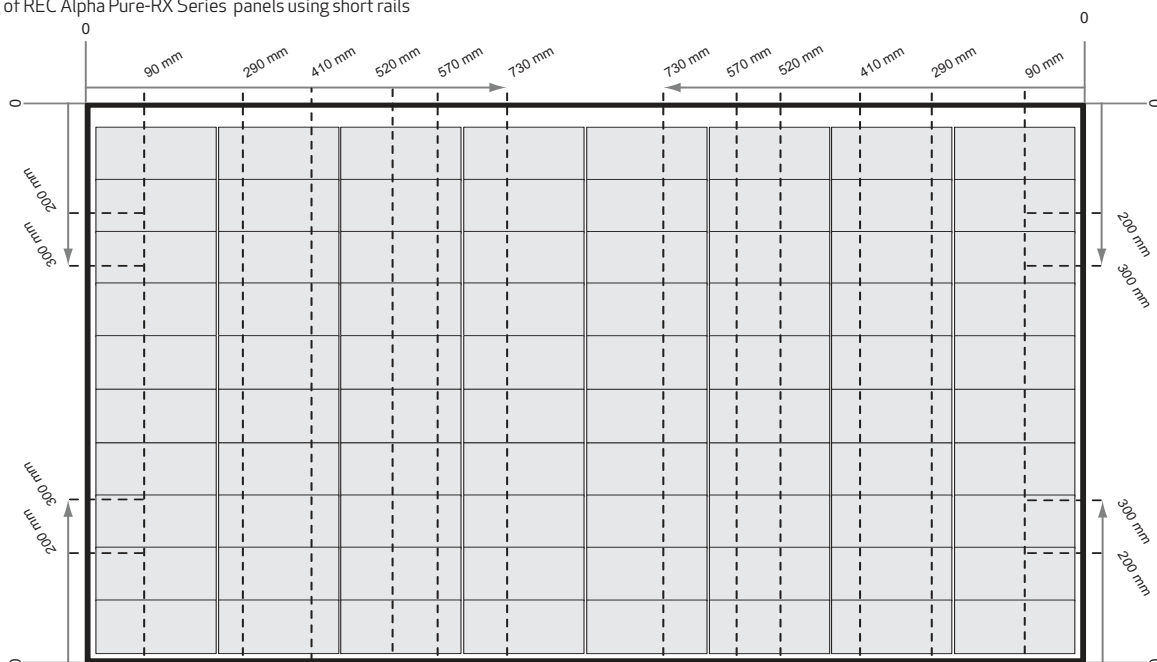
Fig. 11: Clamping of REC Alpha Pure-RX Series panels using short rails
