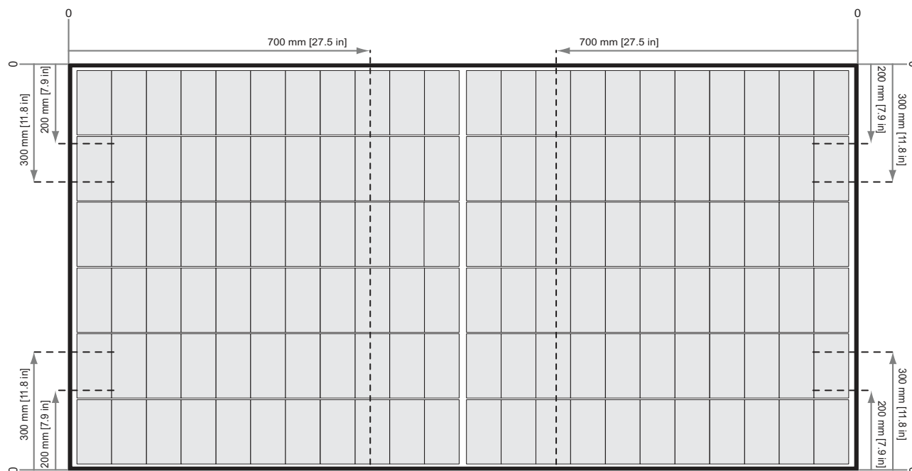
Fig. 4: Clamping of REC Alpha Pure Series panels with rails parallel to long side of the panel
