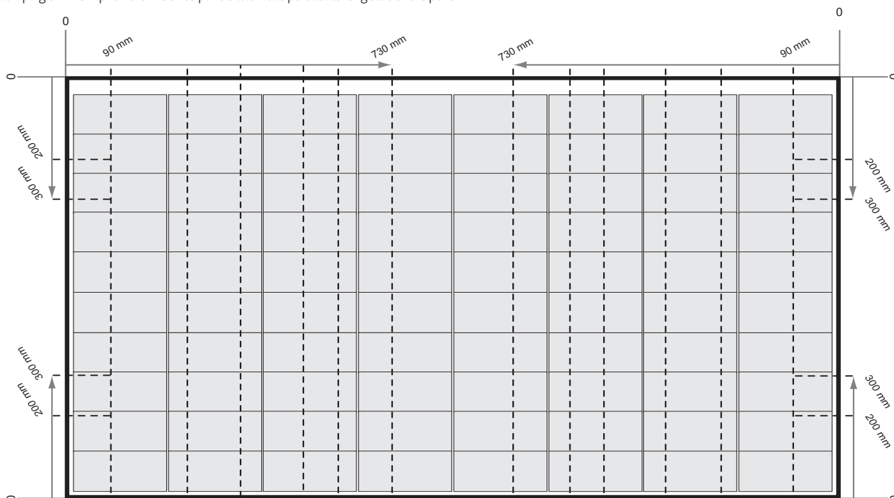
Fig. 7: Clamping of REC Alpha Pure-R Series panels with rails parallel to long side of the panel
