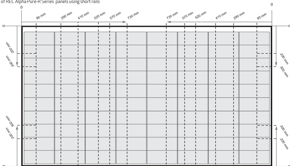
Fig. 8: Clamping of REC Alpha Pure-R Series panels using short rails
