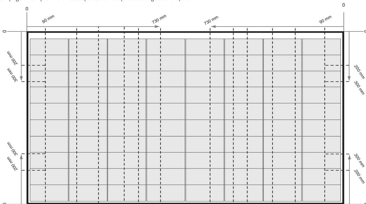
Fig. 10: Clamping of REC Alpha Pure-RX Series panels with rails parallel to long side of the panel
