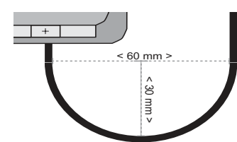
Fig. 18: Minimum cable bend radius
