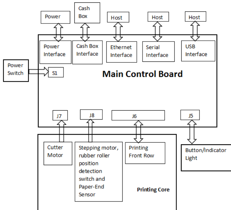
Fig2.2.1 Connection diagram of serial port +USB+ network port control board
