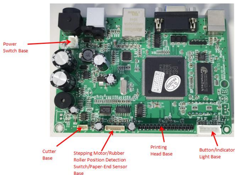
Fig2.2.1 Connection diagram of serial port +USB+ network port control board
