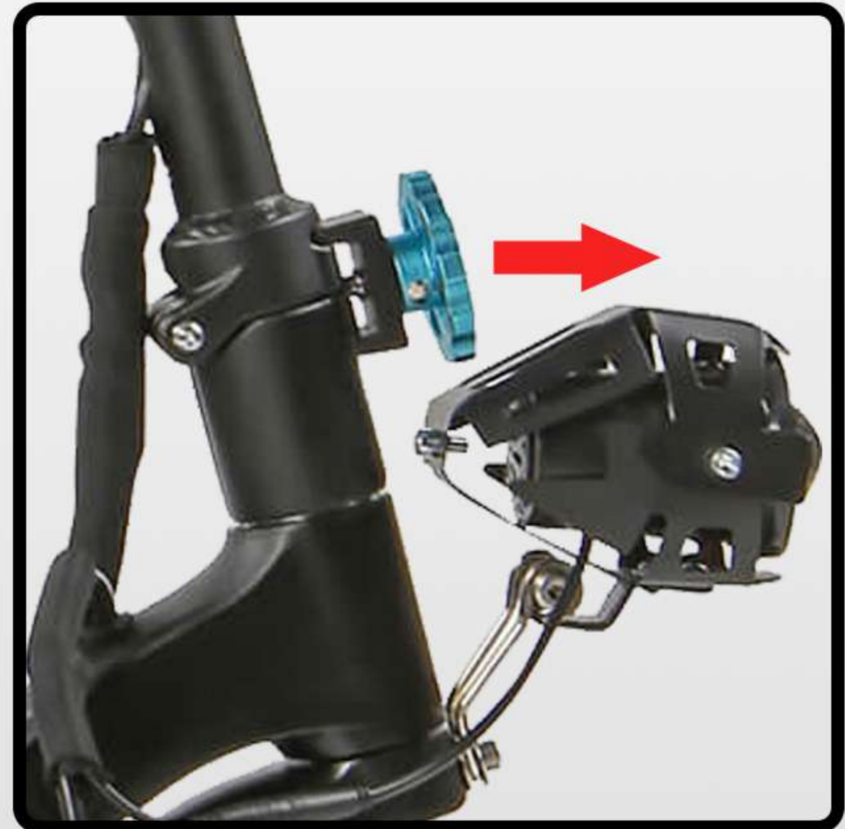
② Keep loosening the folding knob until the J-shaped buckle completely leaves the grooves
