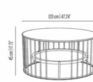
BB_CAG05t_double_D120
