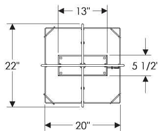
C400FB Cube Chandelier with Flat Box 22" x 22" x 10"
