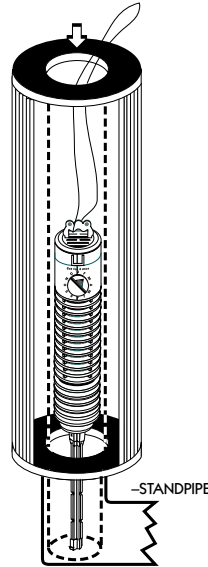
Diagram B - High Flow Spas In Filter Well
