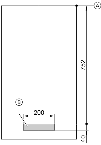
Vitodens 200-W, 49 to 99 kW
