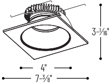
NLCB2-653 6" Cobalt High Lumen Square Reflector with Round Aperture
