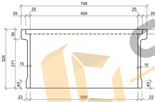
ELEVATION SCALE 1: 10
