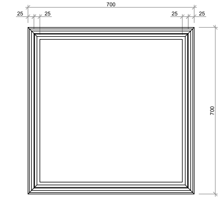
PLAN SCALE 1: 10
