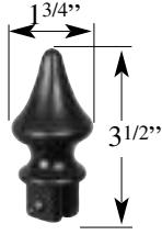
item# TSB3 Finial for Flat Street Blade item# TSB3X Finial for Extruded Street Blade
