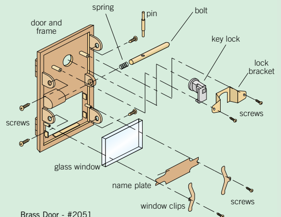
Brass Door - #2051 Rear view of #1 brass door
