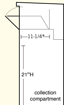
3475 (side view)
