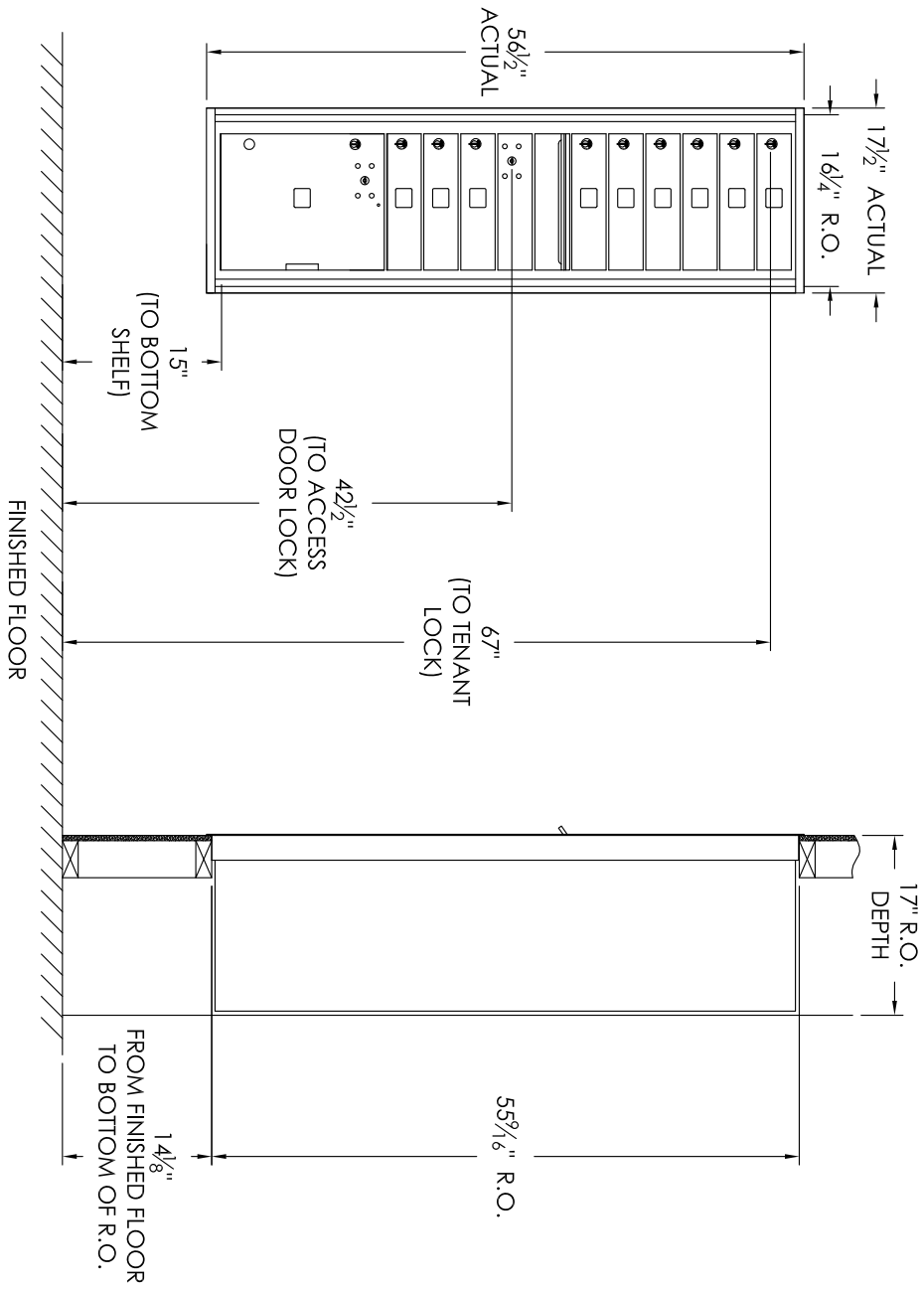
COMPARTMENT CHART
