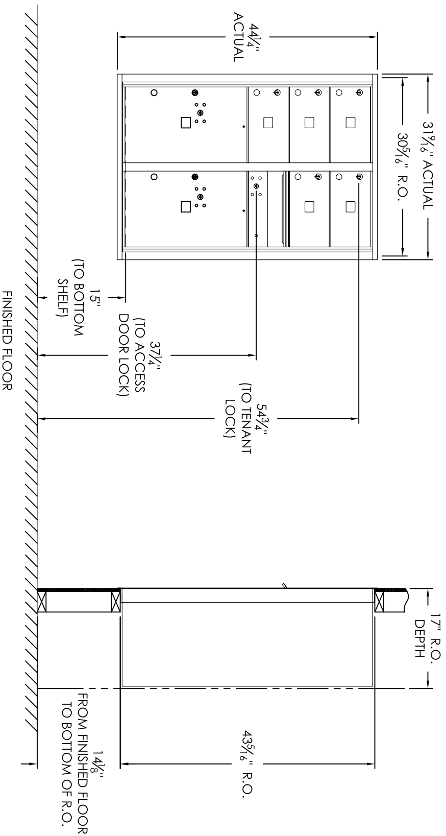
COMPARTMENT CHART
