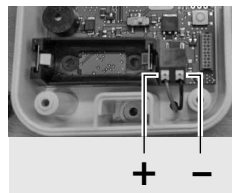
Fig. 2: Power supply connection
