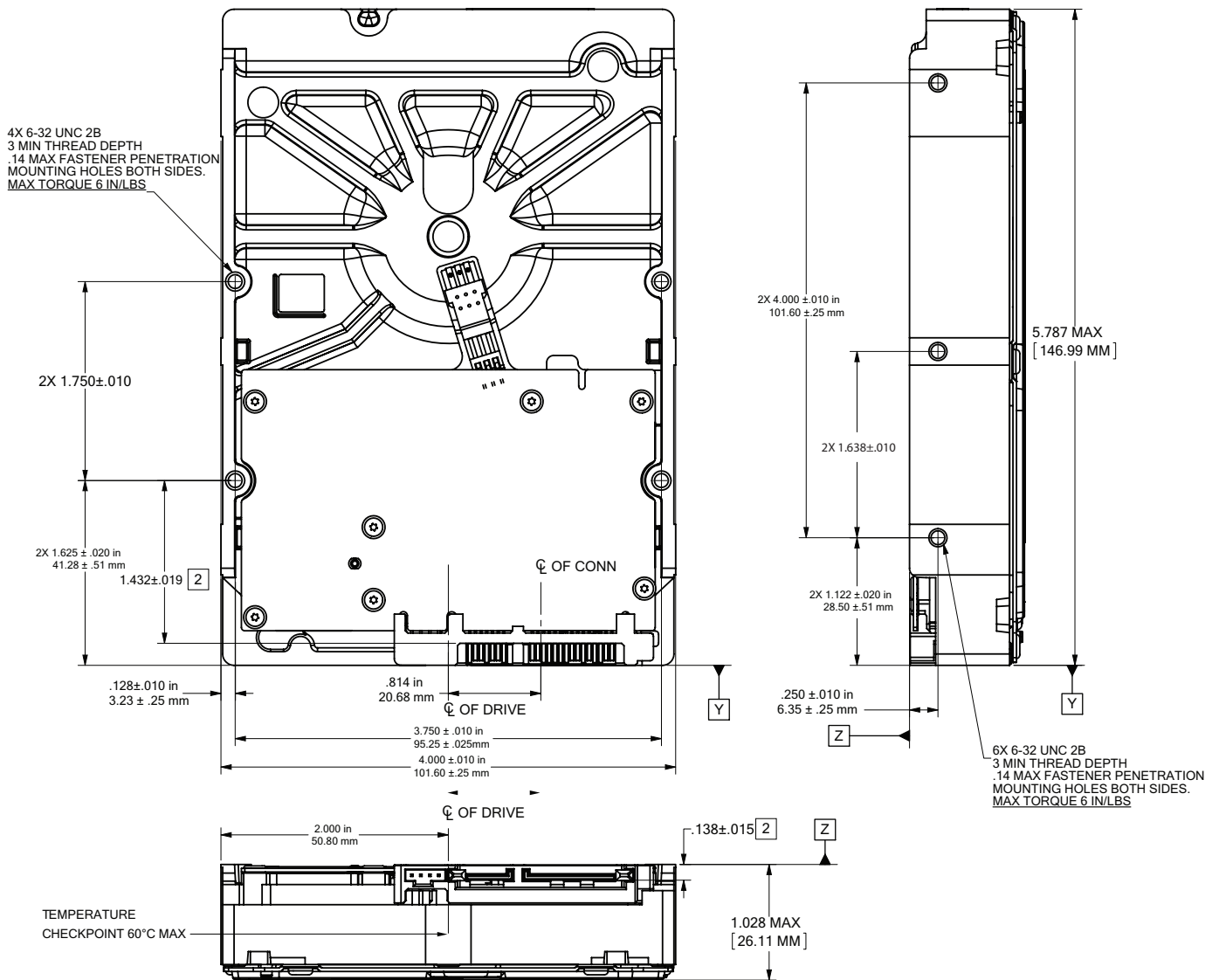
Figure 4 Mounting dimensions (6TB)
