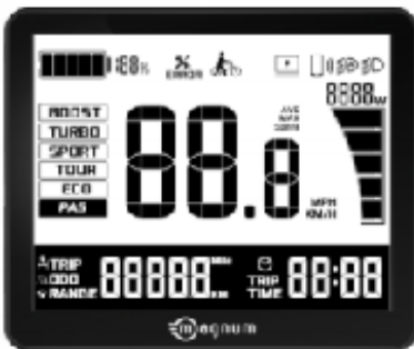
Start-up Screen
