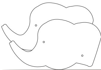
(I) (2 Nos.) Elephant Head Panel
