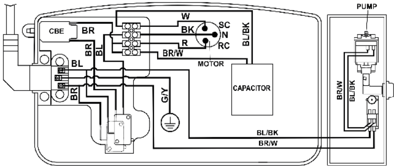
Electrical Layout
