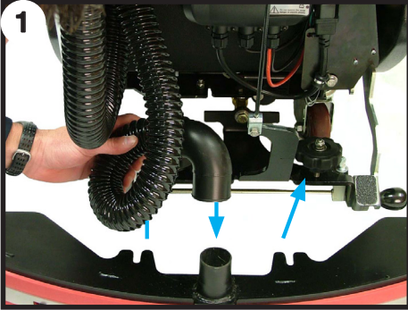
Positioning the squeegee assembly to mount onto the squeegee frame
