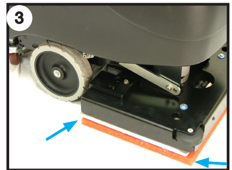
3 Proper alignment of pad
