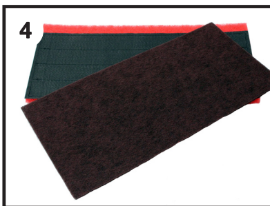
4 Red backer pad & Velcro pad retainer (black) alignment shown above with surface prep pad (brown) pulled away
