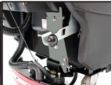
Low down pressure setting
