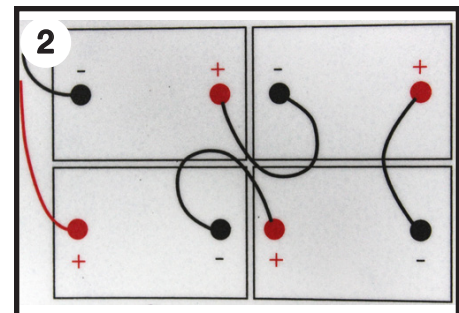
Battery Connection Diagram
