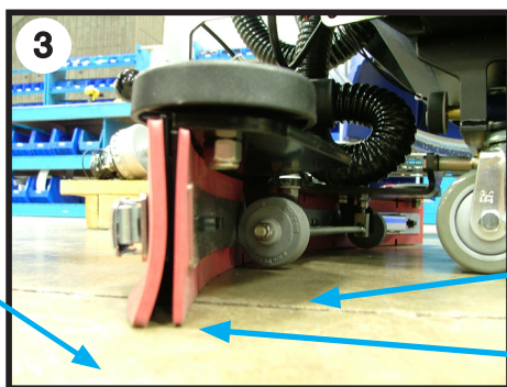
Close up of squeegee assembly and blade deflection
