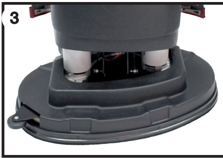
Self-adjusting head shroud with bristle skirt
