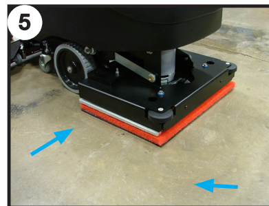
5 Proper alignment of pad
