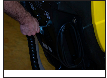
Lowering the squeegee assembly
