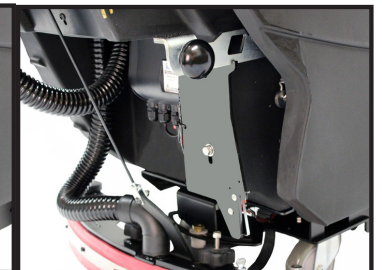
Locking in high down pressure setting by lifting foot lever
