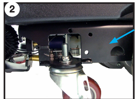
Tie down location on main frame
