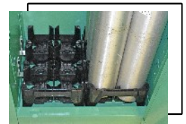
Non Sparking Dividers Hold Cylinders Upright
