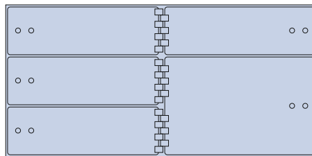
SDXL-5R (Wt. 180 lbs.) 4 openings ea. 5" x 15" and 1 opening ea. 10" x 15"
