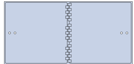
SDXL-2 (Wt. 155 lbs.) 2 openings ea. 15" x 15"
