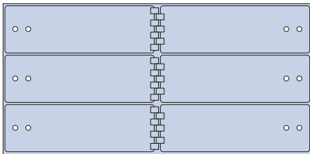
SDXL-6 (Wt. 190 lbs.) 6 openings ea. 5" x 15"
