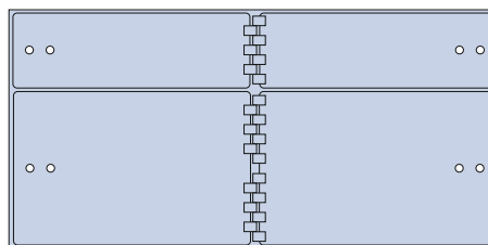
SDXL-4 (Wt. 180 lbs.) 2 openings ea. 5" x 15" and 2 openings ea. 10" x 15"
