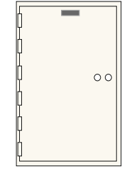
SDXN-1 (55 lbs.) 1 opening ea. 15" x 10"
