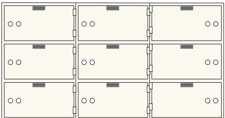
SDX-9 (160 lbs.) 9 openings ea. 5" x 10"
