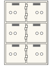
SDXN-6 (70 lbs.) 6 openings ea. 5" x 5"
