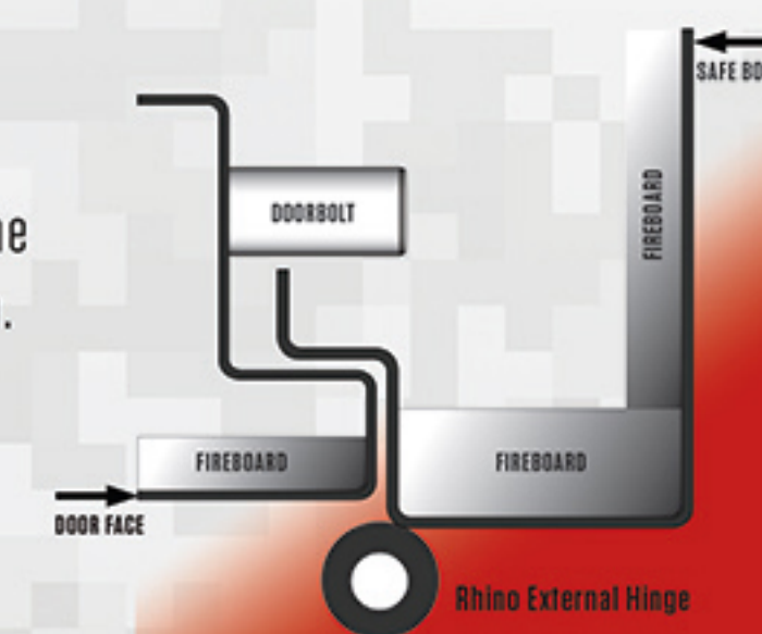
Rhino Door Construction
