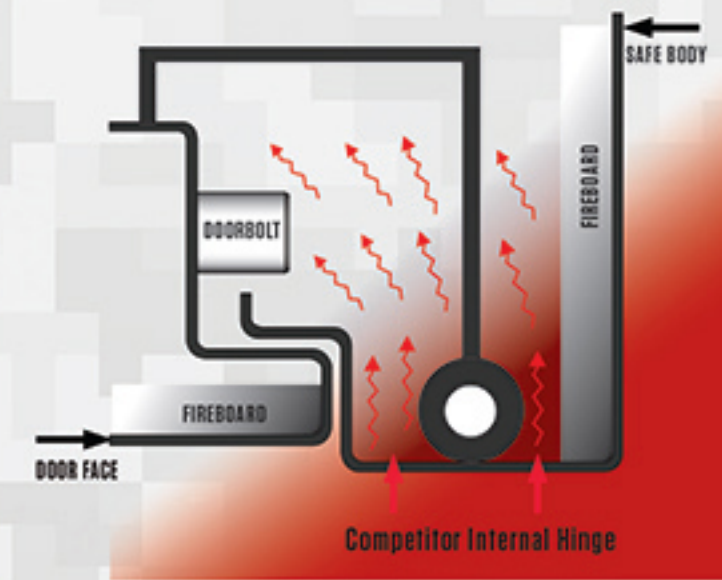
Competitor's Door Construction
