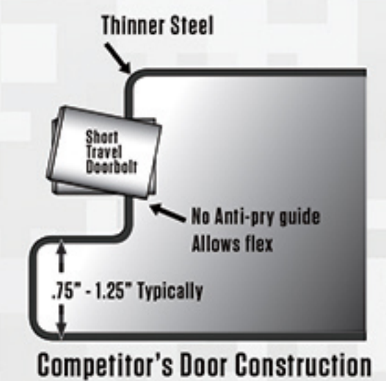
Competitor's Door Construction
