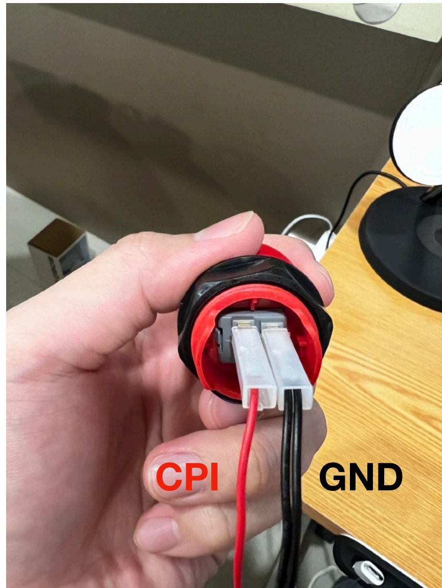
Connect CPI and GND PIN with a button
