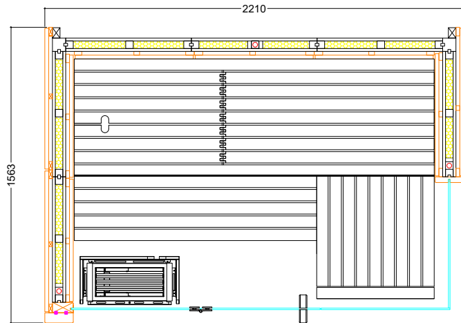
assembly left
