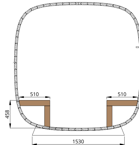
section (terrace)
