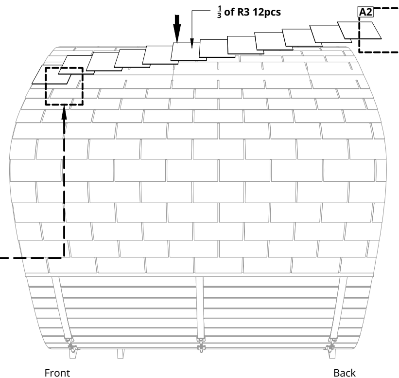
Dice Sauna (COMFY2.4)
