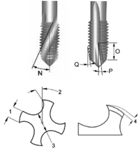
Spiral Flute Tap Spiral Point Tap
