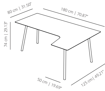
MAAA180_ table 180x80 | 70 55 / 64 " x 31 1 / 2 " return table
