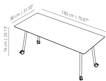
MAA180_ table 180x80 | 70 55 / 64 " x 31 1 / 2 " with casters
